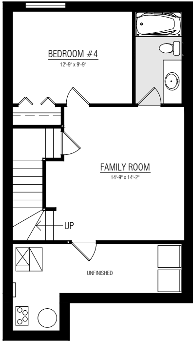
OPTION #1 - 476 SQ.FT.
